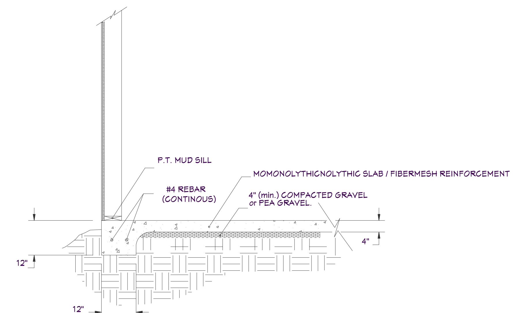
Garage Floor Section
