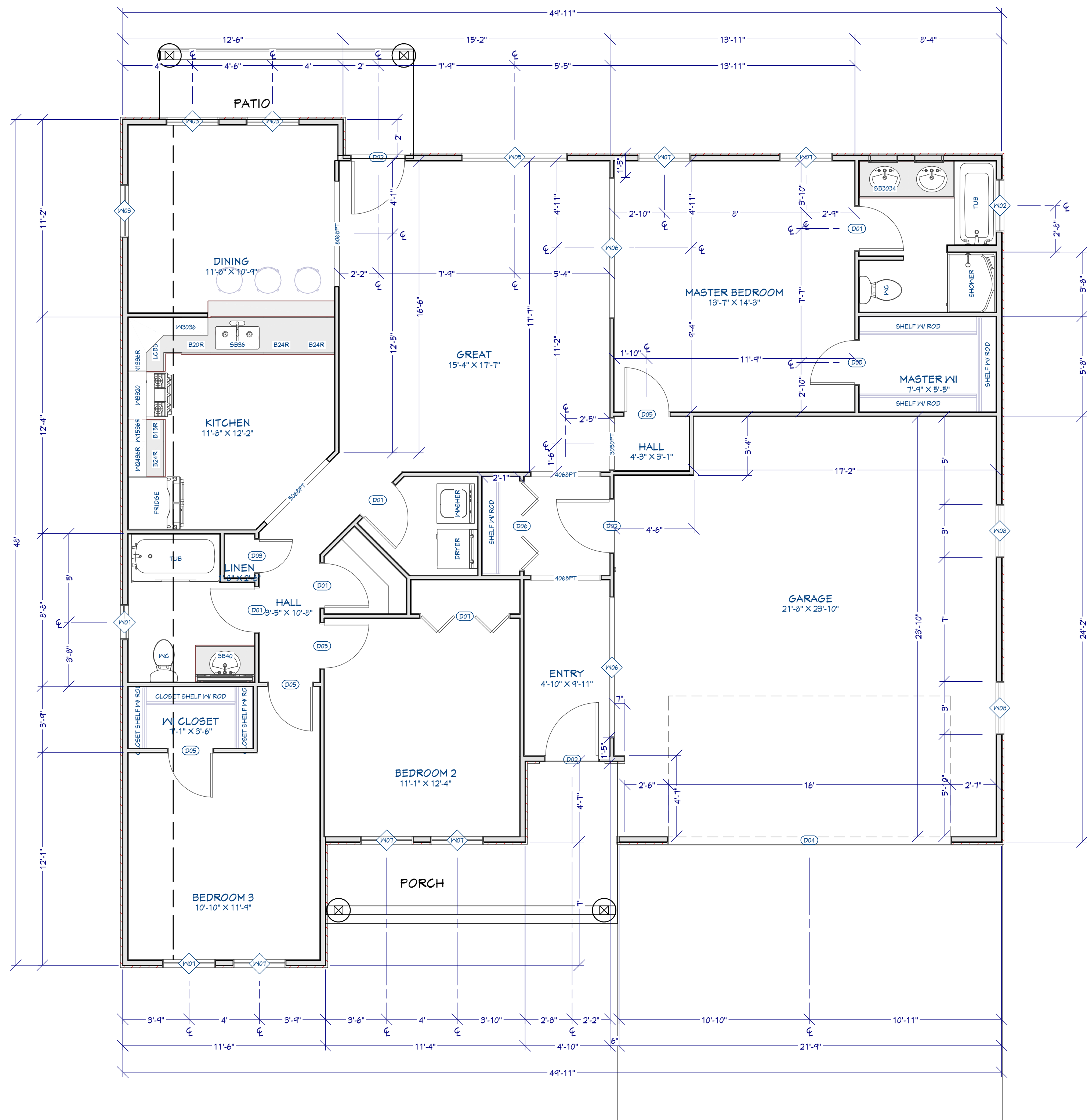
Floor Plan View Dimensioned Scale: 1/4"=1'-0"
