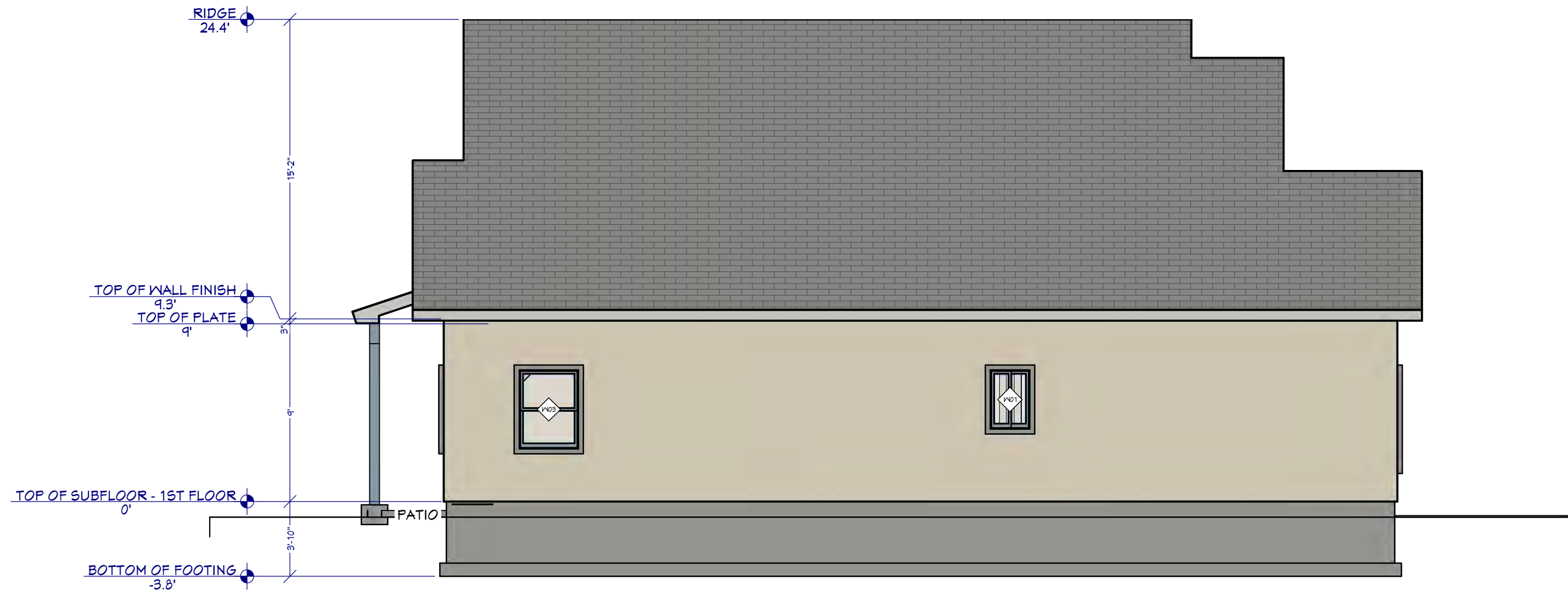
Exterior Elevation Left Scale 3/16"=1'-0"
