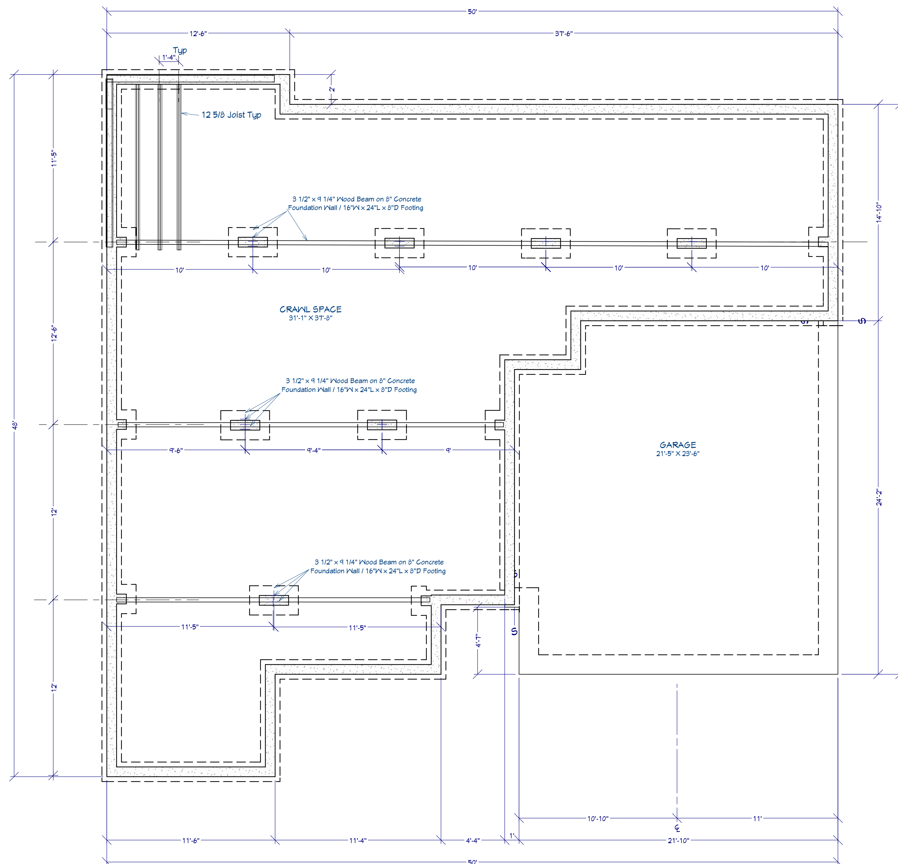
Foundation Plan View Dimensioned Scale: 1/4"=1'-0"
