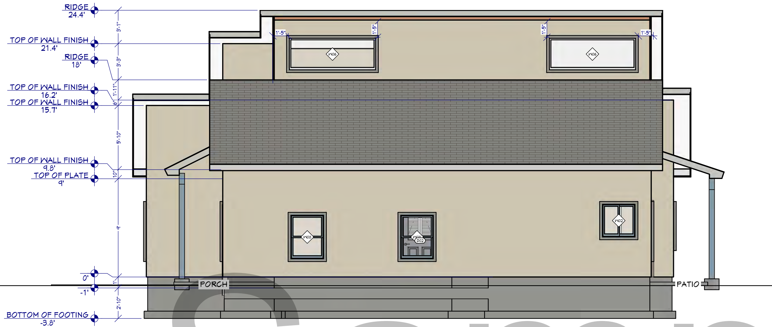
Exterior Elevation Right Scale 3/16"=1'-0"
