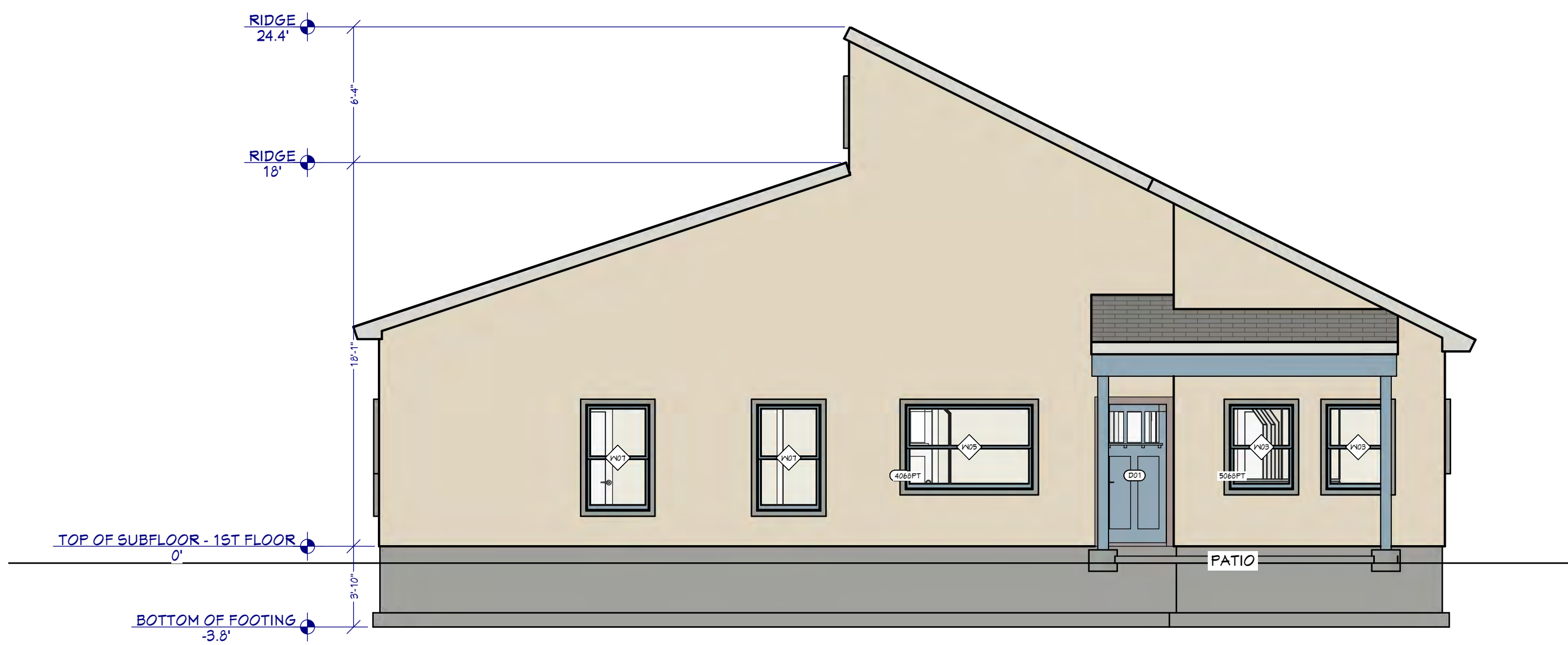
Exterior Elevation Back Scale 3/16"=1'-0"
