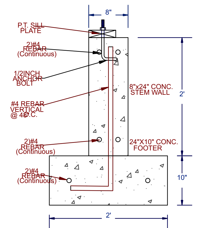
Typical Application around Perimeter Stem Walls
