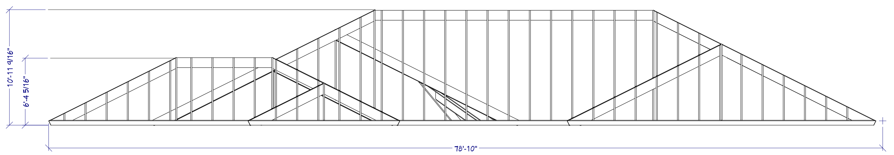
Front View 3/16" = 1'-0"
