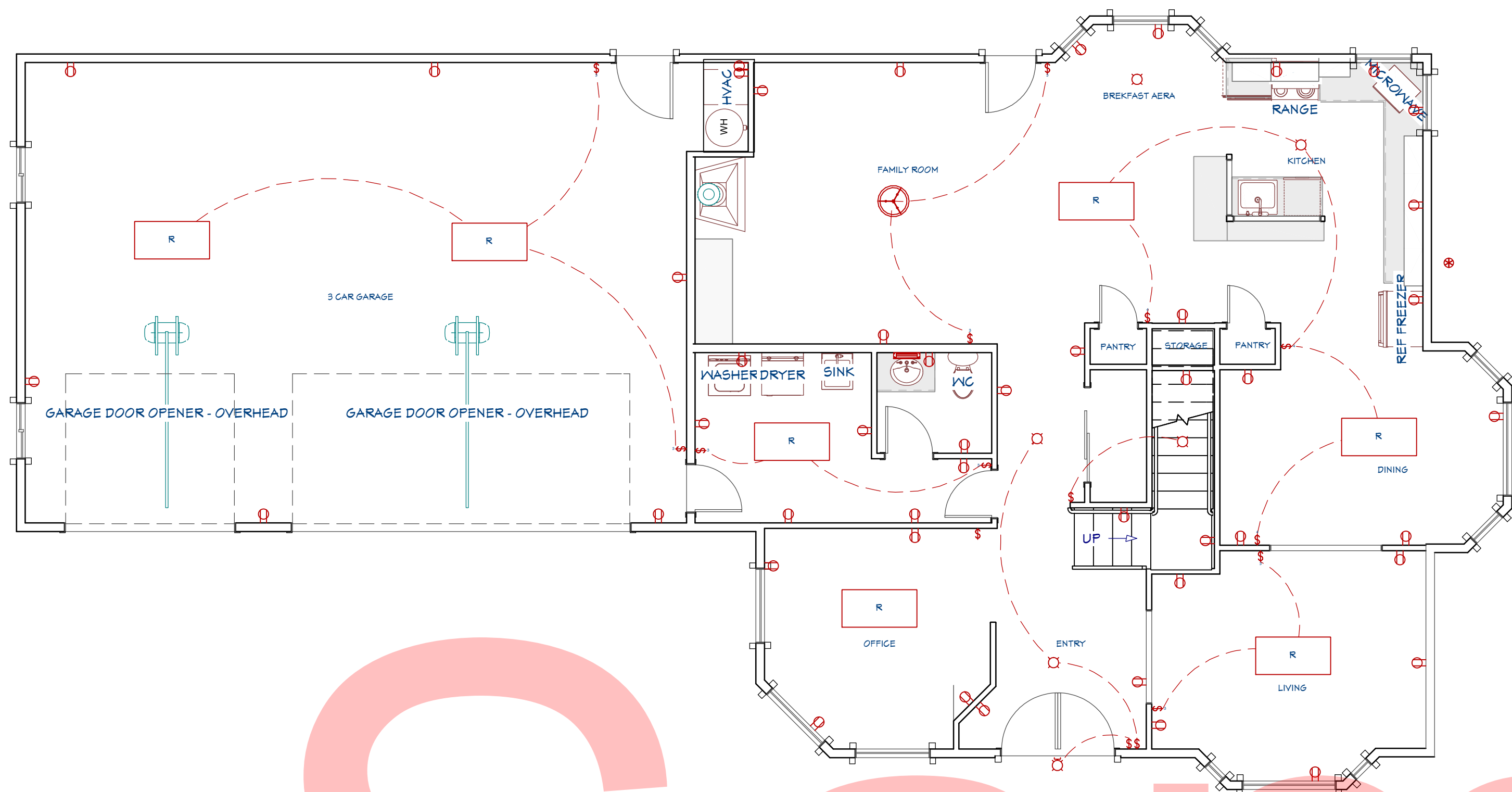
Main Floor Electrical Plan Scale: 3/16" = 1'-0"
