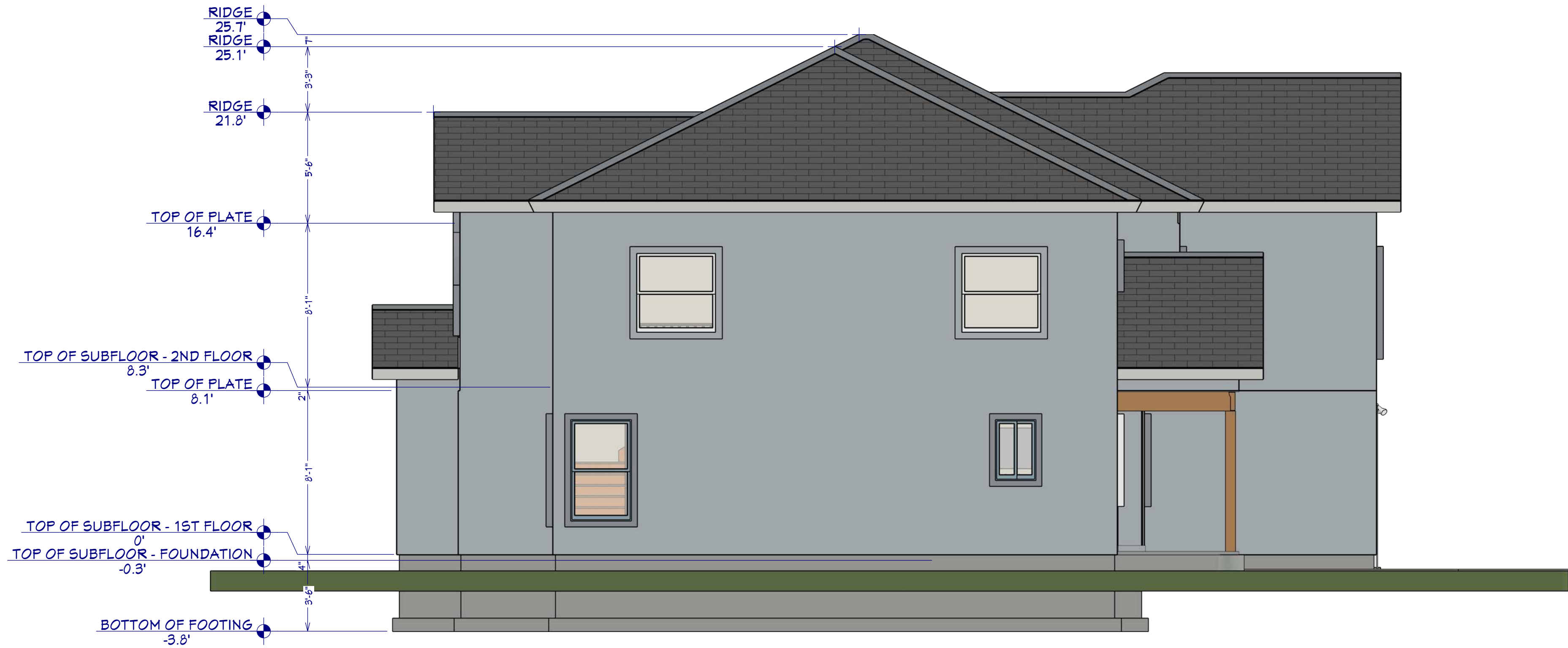
Exterior Elevation Left 1/4"=1'-0"
