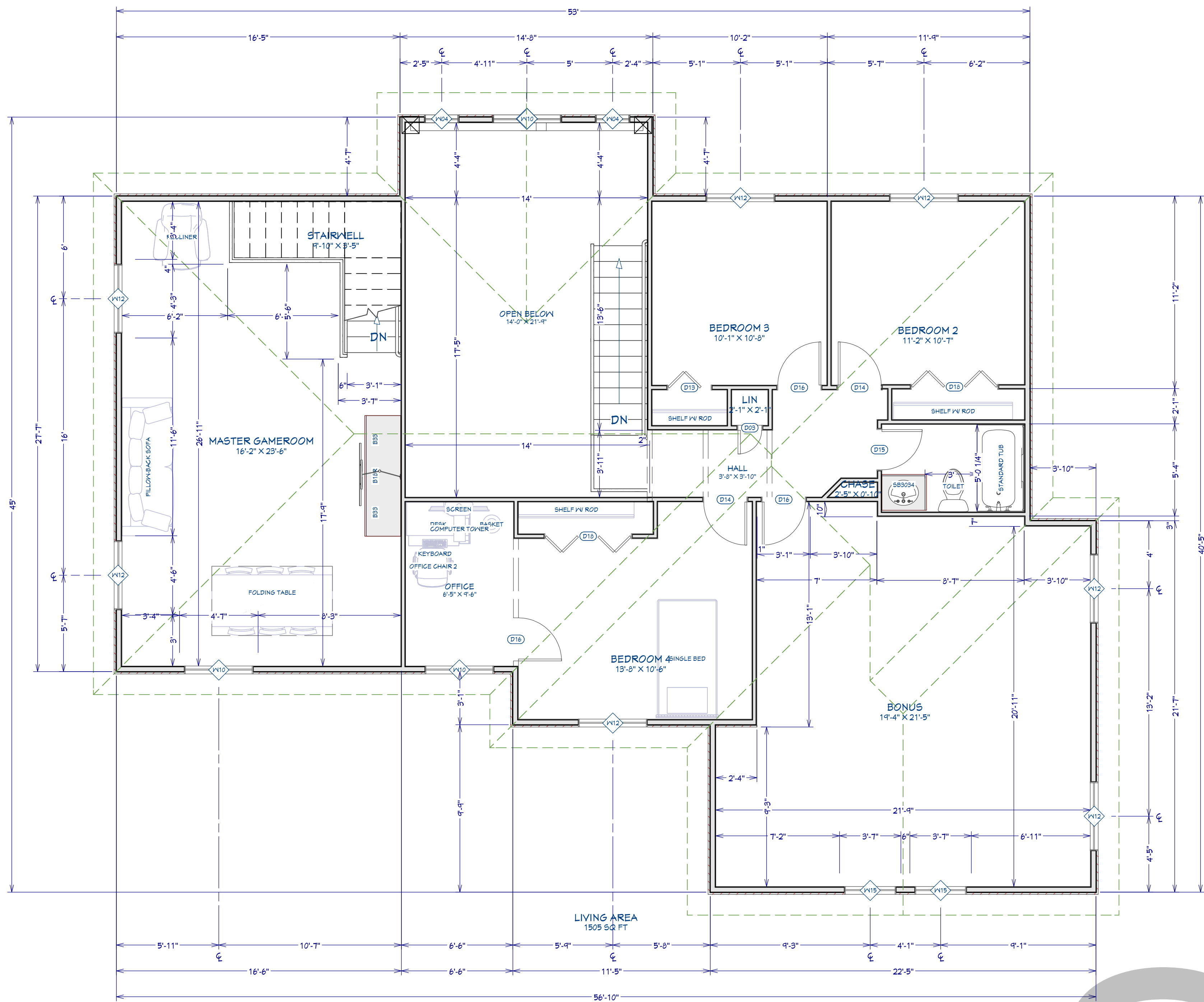
2 nd Floor Plan View Dimensioned 1/4"=1'-0"
