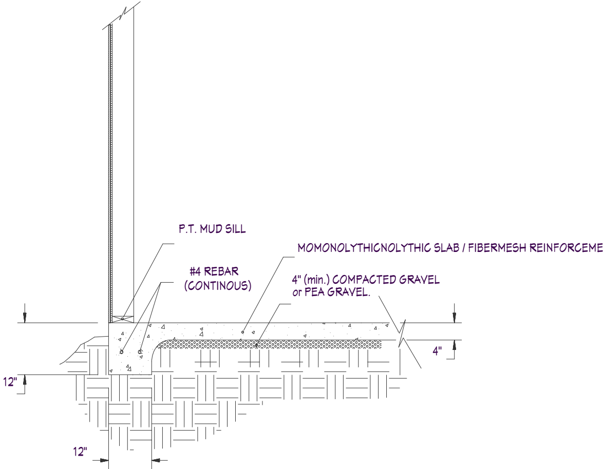
Garage Floor Section
