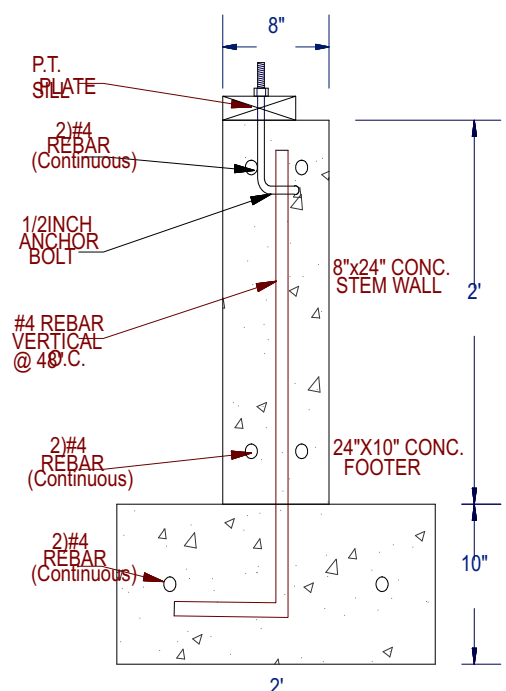
Typical Application around Perimeter Stem Walls
